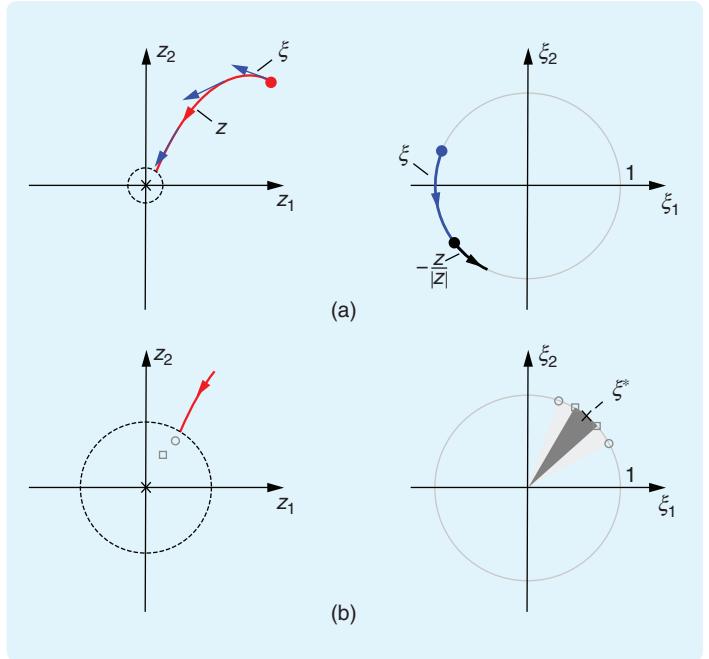
FIGURE 19 Position z = (z_1, z_2) and orientation \xi = (\xi_1, \xi_2) of the mobile robot with hybrid controller in Example 35. (a) The position, orientation, and ratio -z/|z| with the first controller are shown on the z and \xi planes. The position z is in red, the orientation \xi is in blue, and -z/|z| is in black. The first controller drives z to a neighborhood of z = 0 and \xi to -z/|z| . (b) The second controller drives the orientation to a cone centered at \xi^* with aperture depending on z . Cones associated to two points in a neighborhood of z = 0 are depicted. The two points, indicated by a square and a circle, along with the neighborhood around z = 0 , indicated with dashed line, are depicted in the z plane, while their associated cones are denoted on the \xi plane. As z approaches the origin, the aperture of the cone approaches zero.
