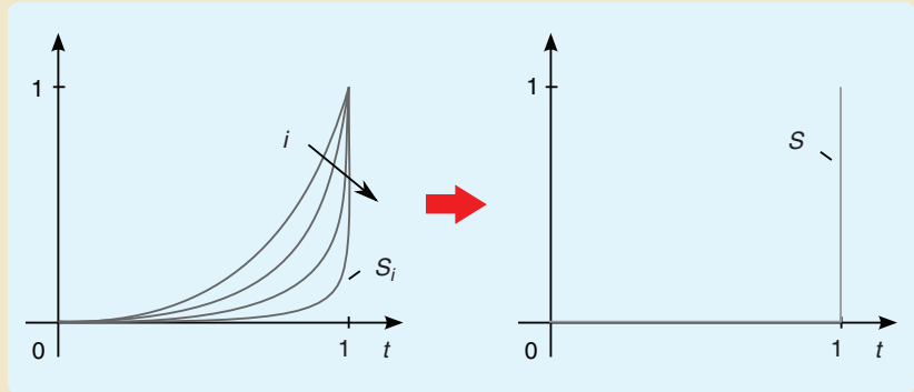
FIGURE S6 A sequence of sets S_j converging to the reflected L-shaped set S . Equivalently, the sequence of functions with graphs given by S_j s converges graphically to a set-valued mapping with graph given by S .
