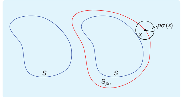
FIGURE 15 Enlargement of a set S due to a state-dependent perturbation of size \rho\sigma . The perturbed set S_{\rho\sigma} contains all points x with Euclidean distance from the unperturbed set S no larger than \rho\sigma(x) .
