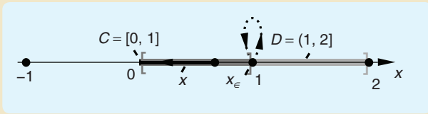
FIGURE S9 The effect of state perturbations in Example S7 showing that the global asymptotic stability of the origin is not robust. The solution x starts in (-\infty, 1) and flows according to the differential equation \dot{x} = -x toward the origin. The solution x_\varepsilon starts at x_\varepsilon(0, 0) = 1 and is obtained under the presence of a perturbation e of size \varepsilon . The perturbation is such that x_\varepsilon(t, j) + e(t, j) \in D for all (t, j) \in \text{dom } x_\varepsilon . Hence, as denoted with dotted line, the solution x_\varepsilon jumps from 1 to 1 infinitely many times, indicating that the origin is not robustly asymptotically stable to small perturbations.
