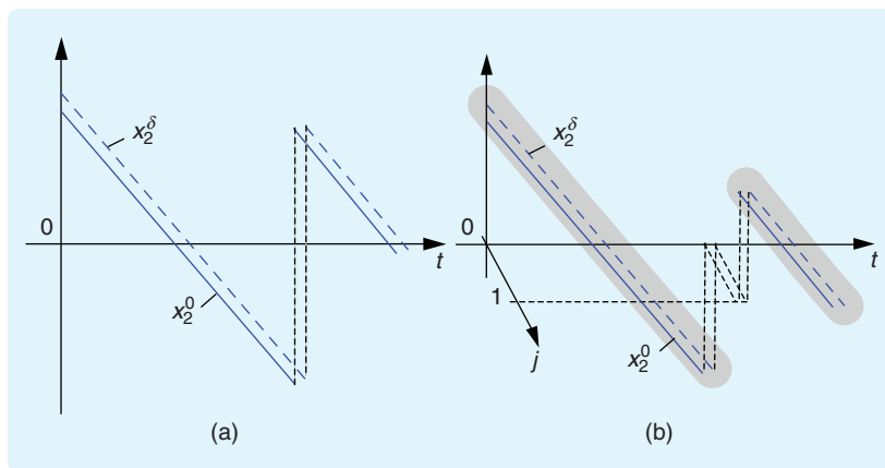
FIGURE 14 Components x_2^\delta, x_2^0 of solutions from “Example 3 Revisited,” representing the velocities of bouncing balls dropped from heights 1 and 1 + \delta , respectively. (a) Velocities parameterized by t . The velocities are not close in the uniform distance since their difference, at times after the first ball bounces and before the second ball bounces, is large. (b) Velocities on hybrid time domains. The shaded neighborhoods of their graphs indicate that the velocities are graphically close.
